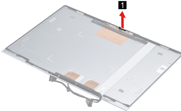
Figure 33. Remove the camera privacy shutter
