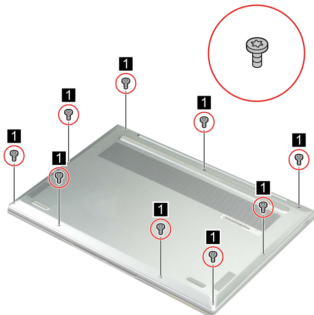
Figure 3. Remove nine screws
