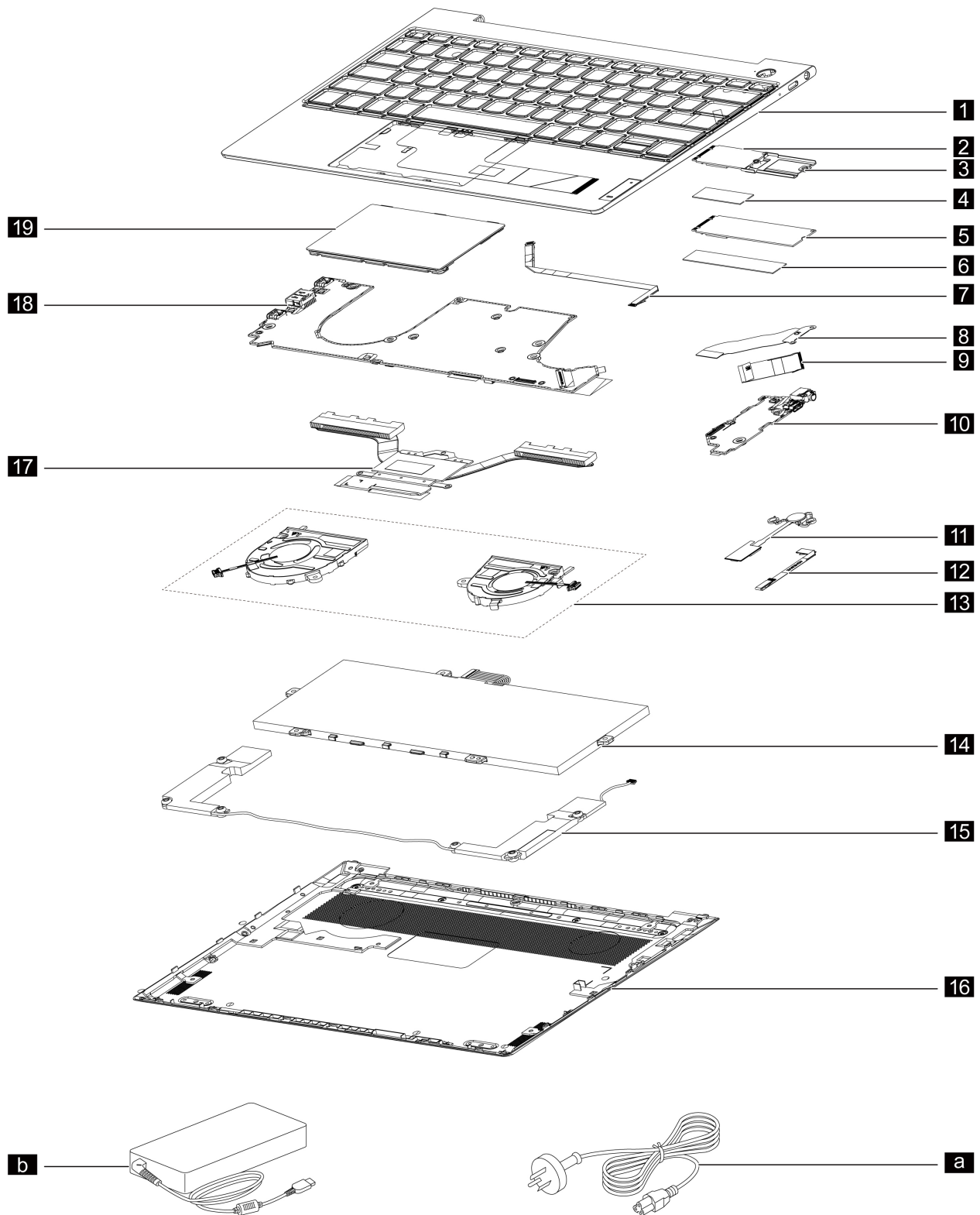
Figure 1. ThinkBook 13x G2 IAP exploded view
