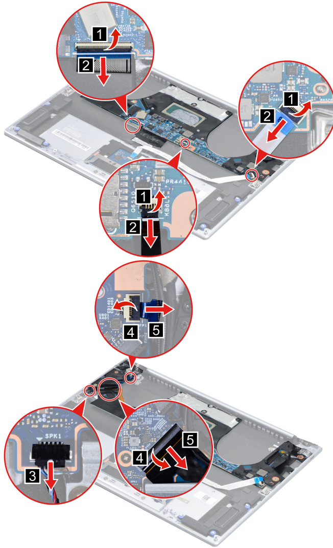
Figure 20. Disconnect cables connected to the system board and USB board
