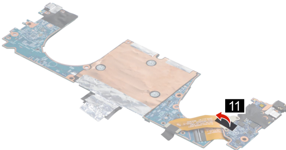
Figure 23. Peel off the tape
