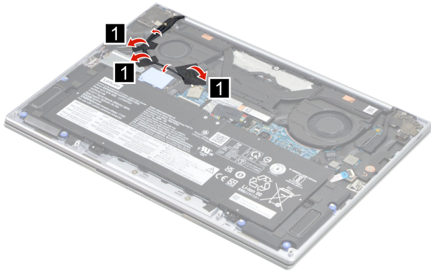
Figure 12. Remove the tape
