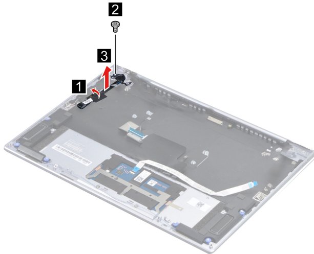
Figure 26. Remove one screw and then remove the fingerprint board and cable
