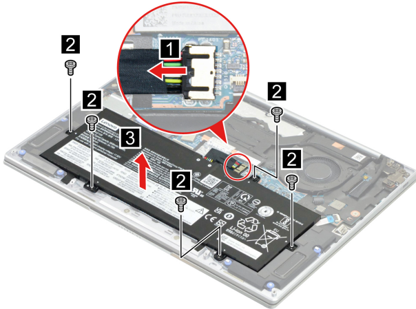
Figure 6. Remove five screws and remove the battery pack
