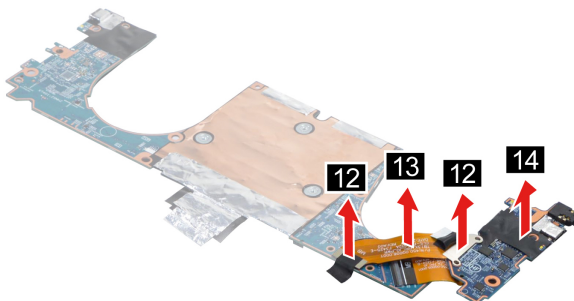
Figure 24. Remove the USB board and cable (70 pin)
