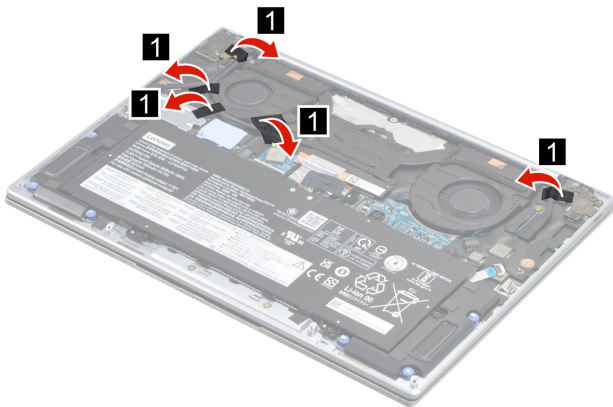
Figure 17. Peel off the tape
