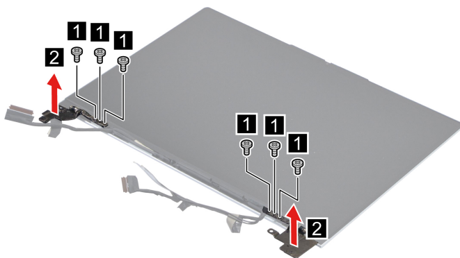
Figure 29. Remove six screws and remove the hinges
