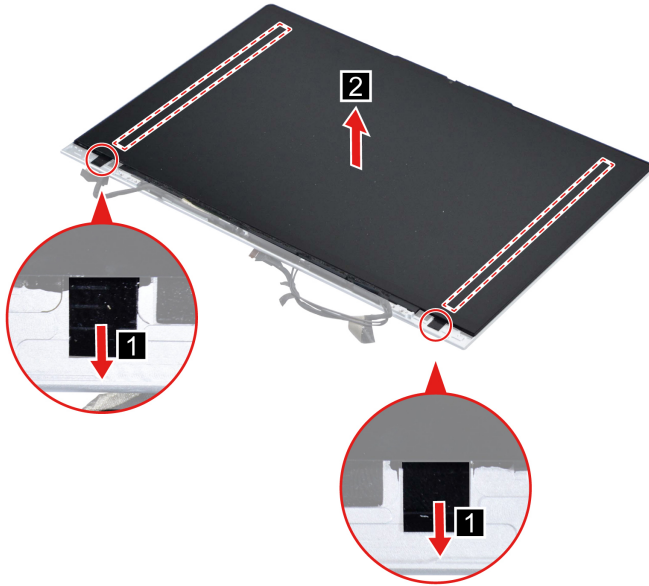
Figure 31. Remove the LCD panel
