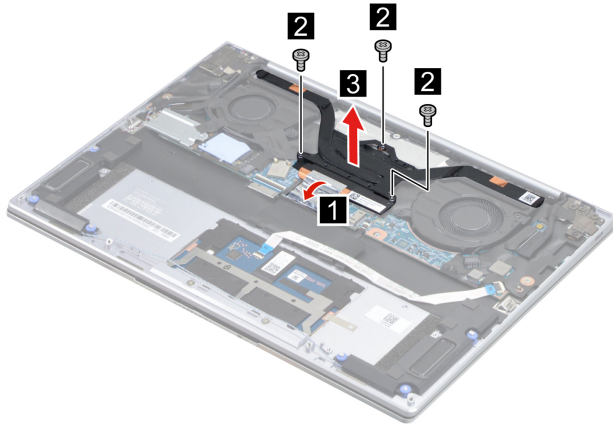
Figure 14. Remove three screws and remove the heat sink
