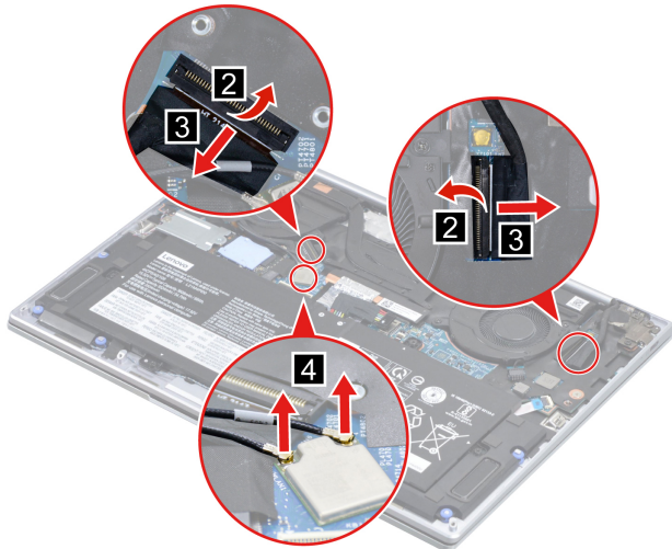
Figure 18. Disconnect the cables
