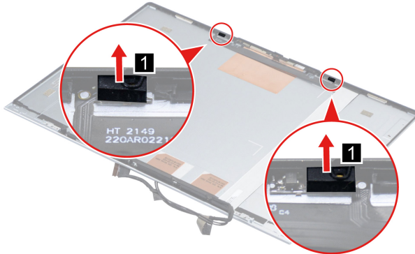
Figure 35. Remove the microphone rubbers
