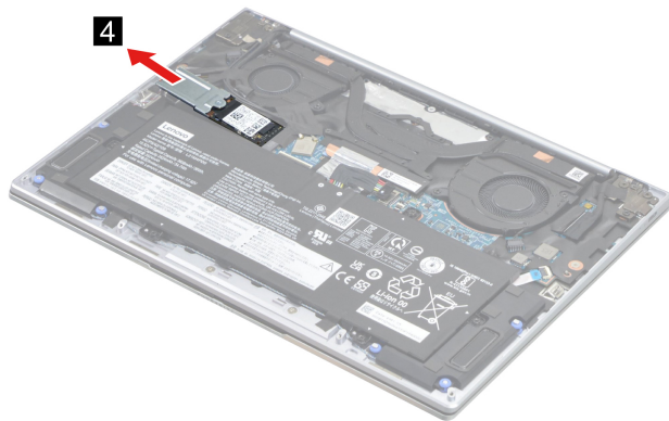
Figure 9. Remove the SSD
