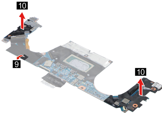
Figure 22. Remove the tape
