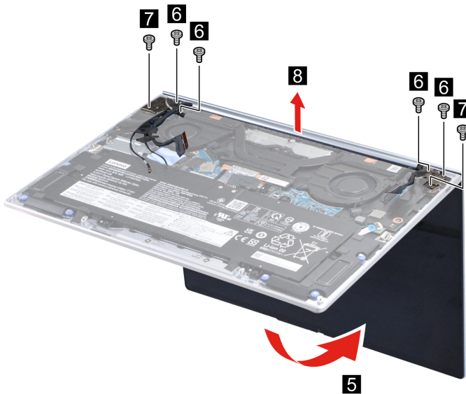
Figure 19. Remove the LCD module
