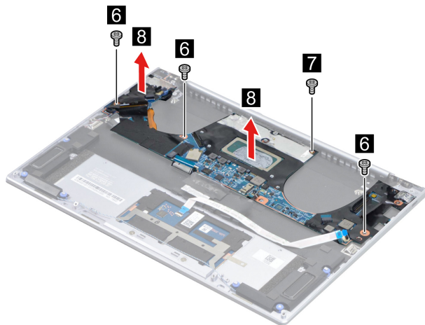
Figure 21. Remove four screws and then remove the system board and USB board.
