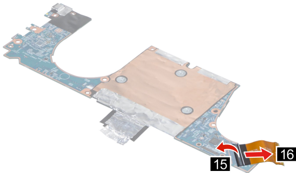
Figure 25. Remove the USB board cable (48 pin)
