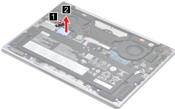
Figure 7. Remove the thermal pad
