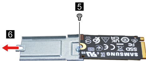
Figure 10. Remove the SSD bracket
