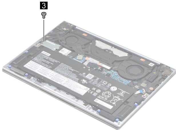
Figure 8. Remove one screw
