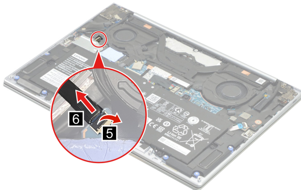
Figure 5. Detach the wireless charging cable connector
