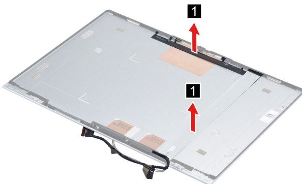
Figure 36. Remove the D-microphone cable
