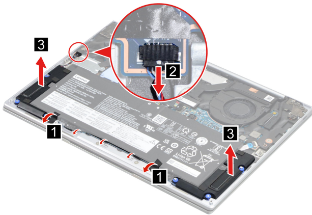
Figure 11. Remove the speakers
