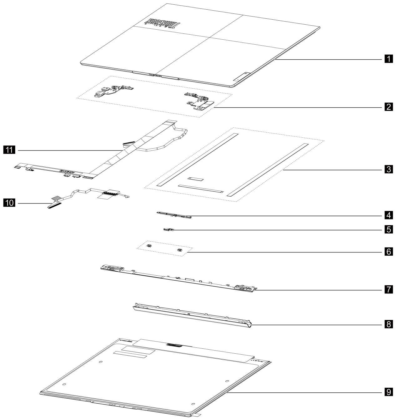
Figure 2. ThinkBook 13x G2 IAP LCD module - exploded view
