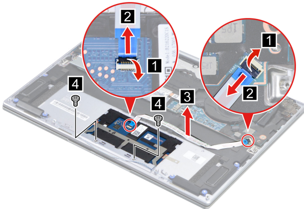
Figure 15. Remove the touchpad cable and two screws
