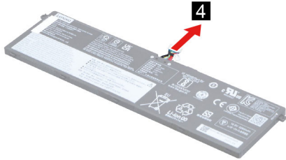
Figure 6. Remove the battery pack cable
