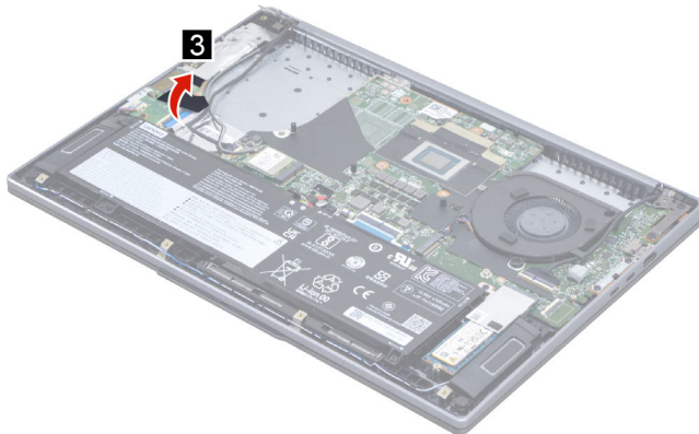
Figure 17. Peel back the I/O board mylar
