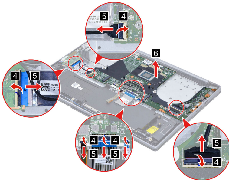
Figure 23. Remove the system board
