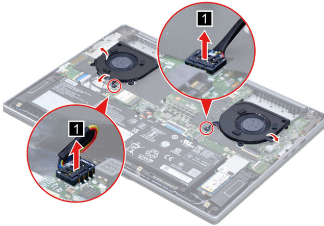
Figure 14. Detach the fan cable connectors and release cables
