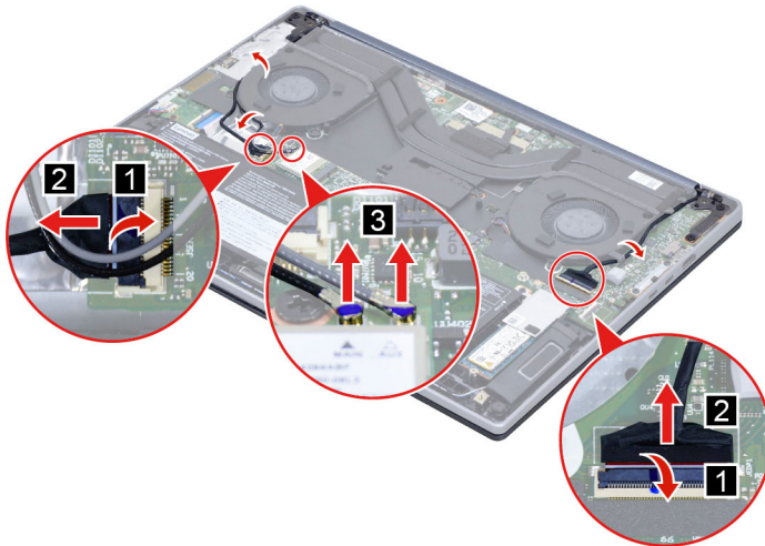
Figure 25. Disconnect the antenna cables, EDP cable and camera cable
