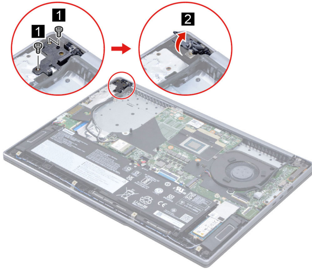
Figure 16. Remove two screws and then open the hinge
