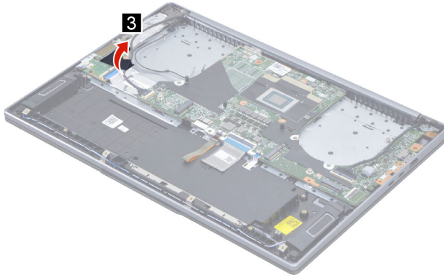
Figure 22. Peel back the I/O board mylar
