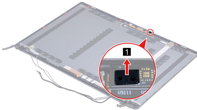
Figure 33. Remove the ToF rubber
