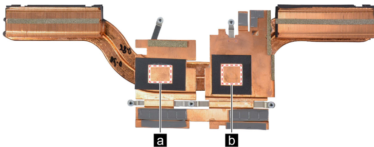
Figure 13. The areas where the thermal interface material should be applied
