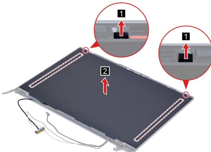
Figure 30. Remove the LCD panel
