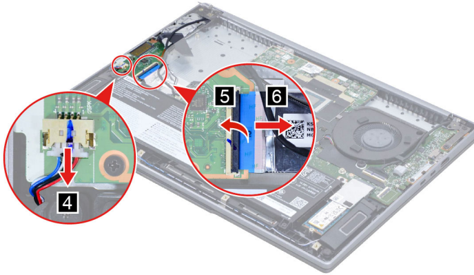
Figure 18. Disconnect cables connected to the I/O board
