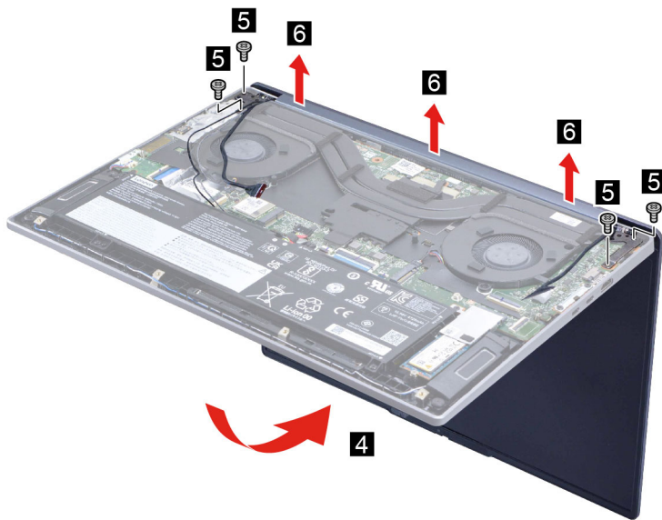
Figure 26. Remove the LCD module
