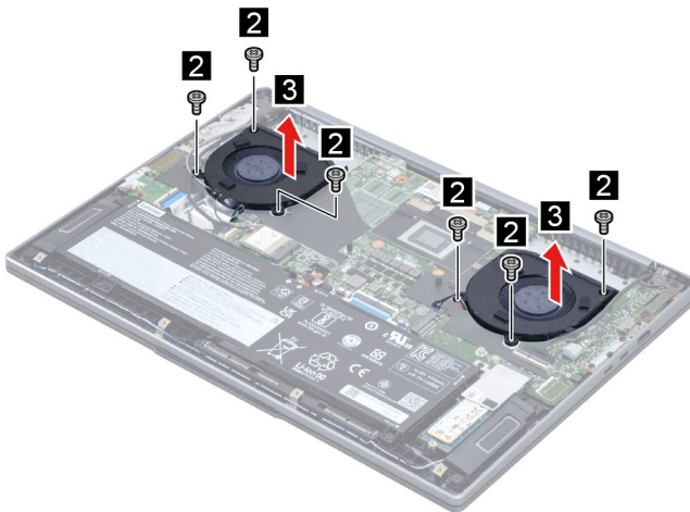
Figure 15. Remove the fans
