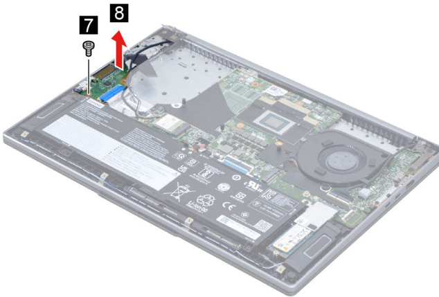
Figure 19. Remove the I/O board
