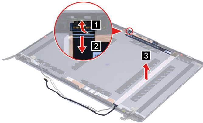
Figure 34. Remove the camera cable
