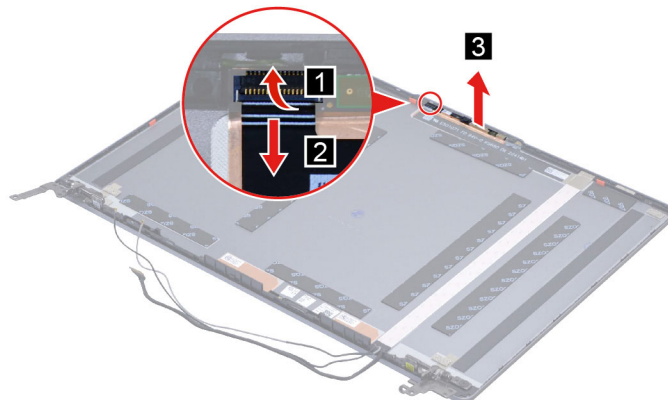
Figure 35. Remove the camera board
