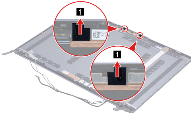
Figure 32. Remove the microphone rubber
