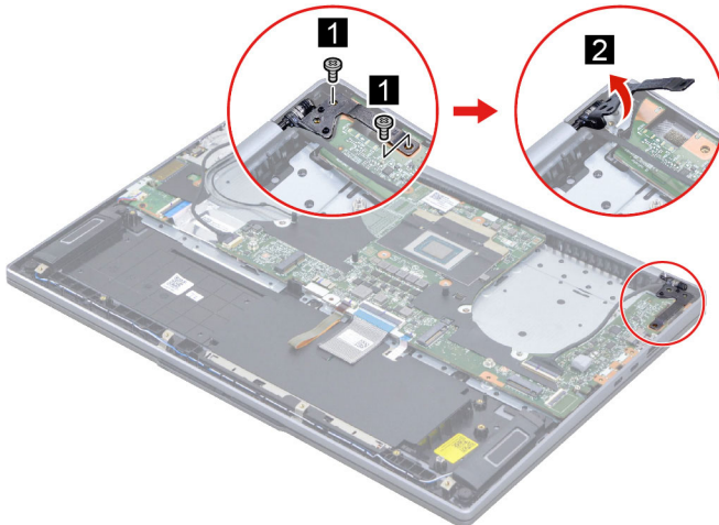
Figure 21. Open the hinge
