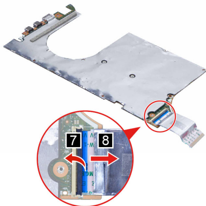
Figure 24. Remove the I/O board cable
