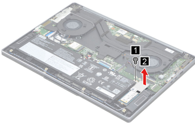
Figure 7. Remove the SSD plate
