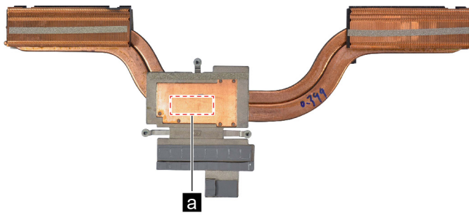
Figure 12. The area where the thermal interface material should be applied
