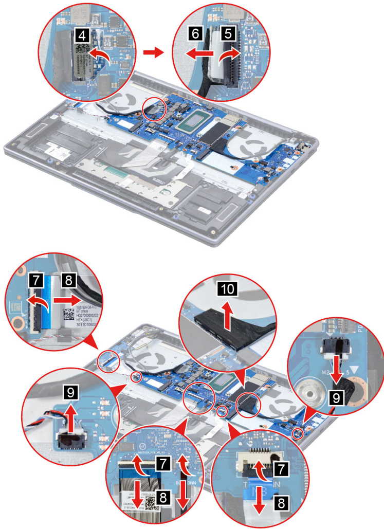
Figure 26. Disconnect cables
