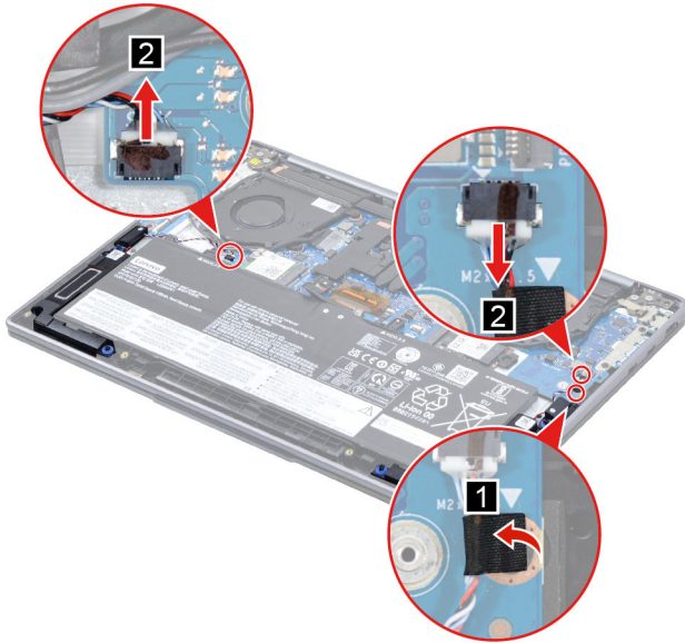
Figure 12. Detach the speaker cable connectors
