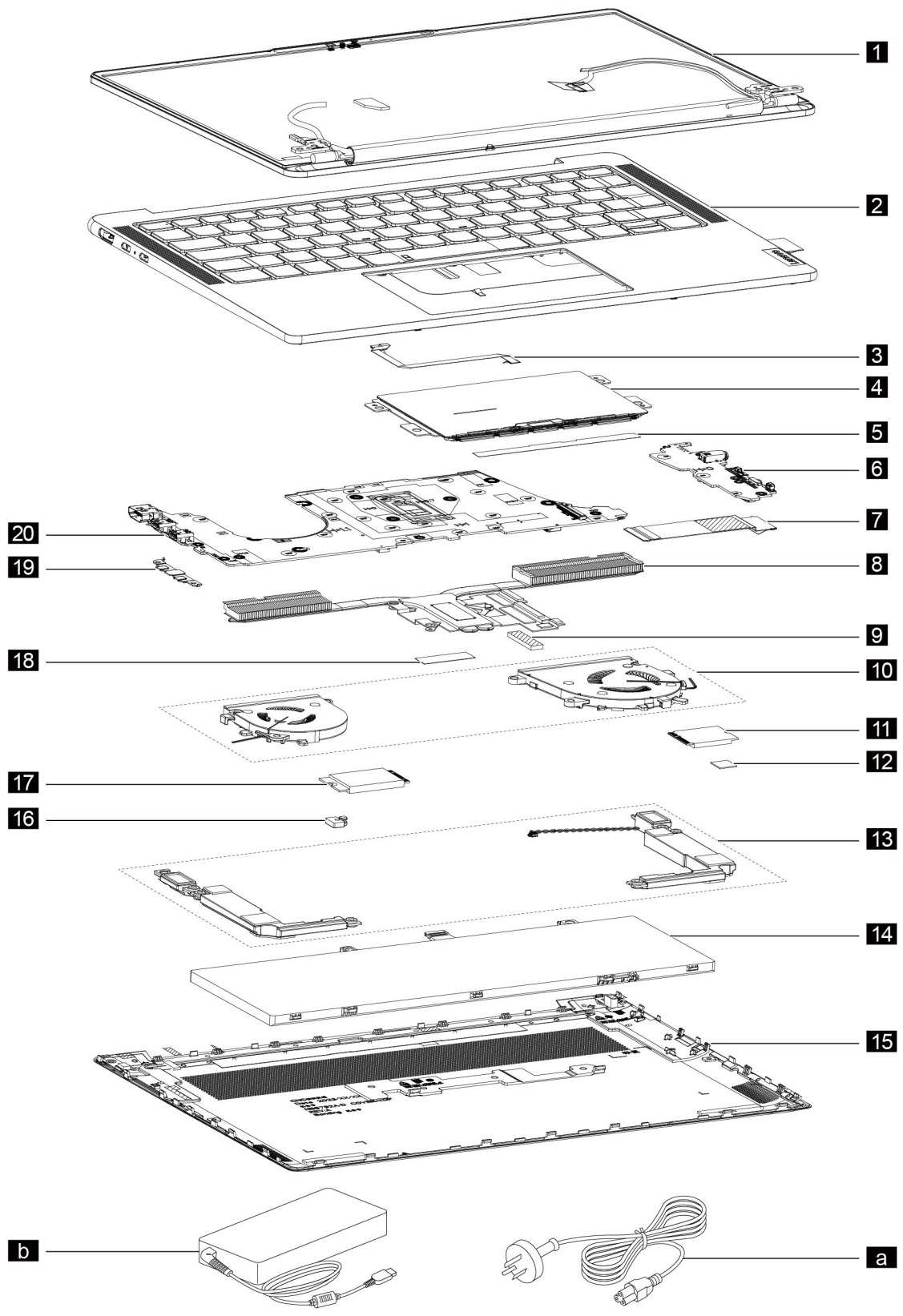
Figure 1. exploded view
