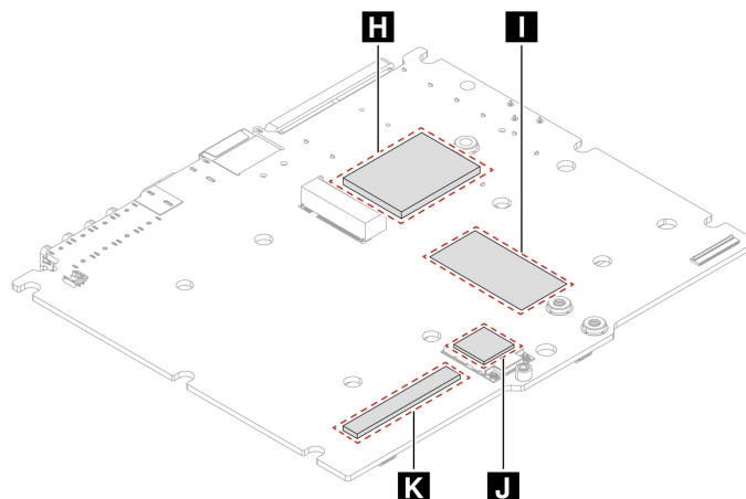
Figure 3. System board surface areas requiring TIM removal prior to reinstallation
