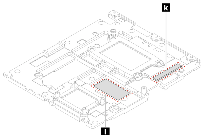
Figure 4. Designated TIM application areas on the stiffener
