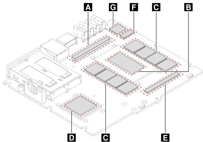
Figure 1. Designated TIM application areas on the heat sink
