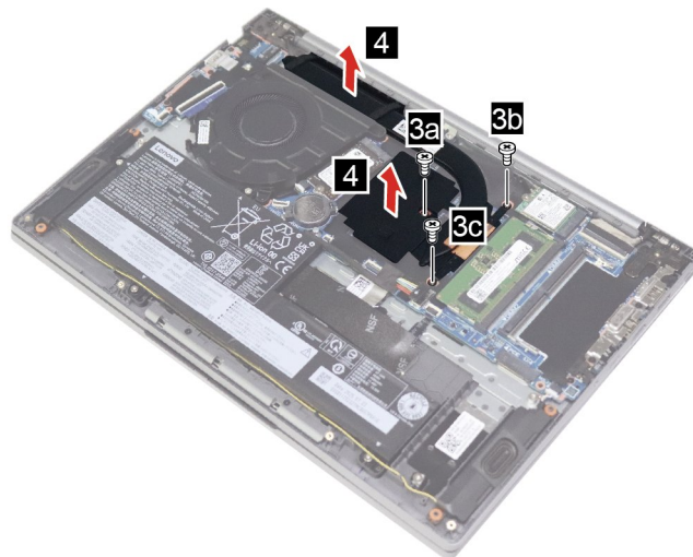
Figure 14. Remove three screws and the heat sink
