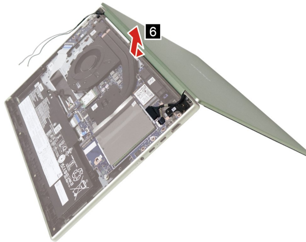
Figure 42. Rotate the LCD/OLED module and remove the LCD/OLED module
