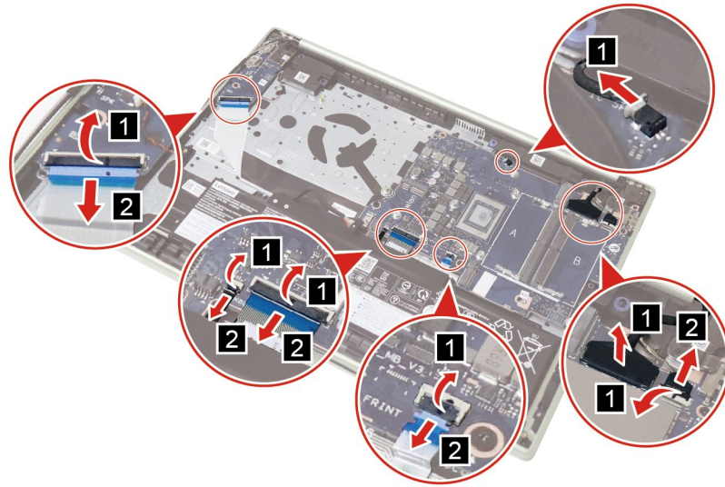
Figure 29. Disconnect cables
