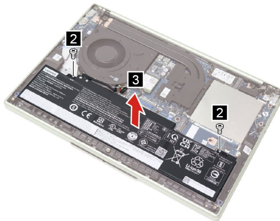
Figure 5. Remove two screws and the battery pack
