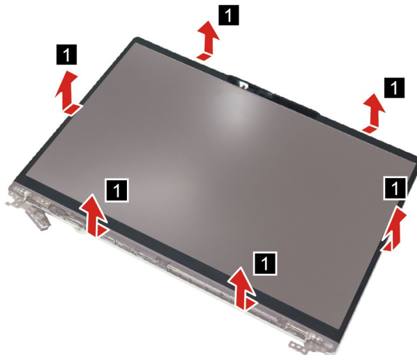
Figure 44. Remove the LCD/OLED bezel
