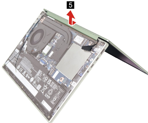
Figure 39. Rotate the LCD/OLED module and remove the LCD/OLED module
