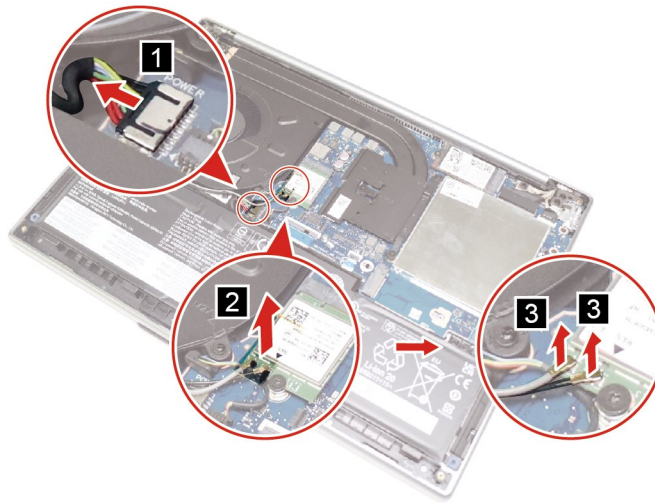
Figure 7. Disconnect the battery pack cable, remove the mylar, and disconnect the antennas
