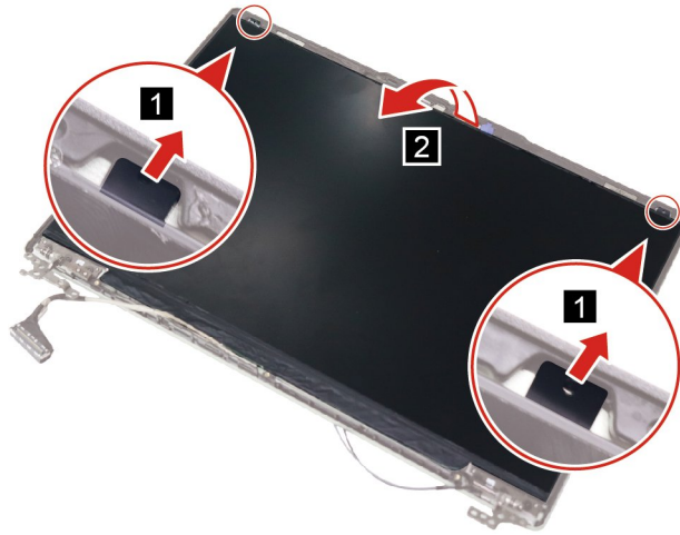
Figure 51. Detach two pieces of stretch-release tape and turn over the LCD panel
