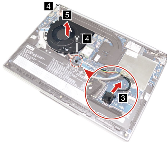
Figure 19. Disconnect the fan cable, remove two screws, and remove the fan
