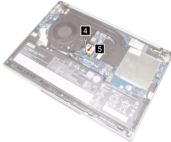
Figure 8. Remove one screw and the Wi-Fi card
