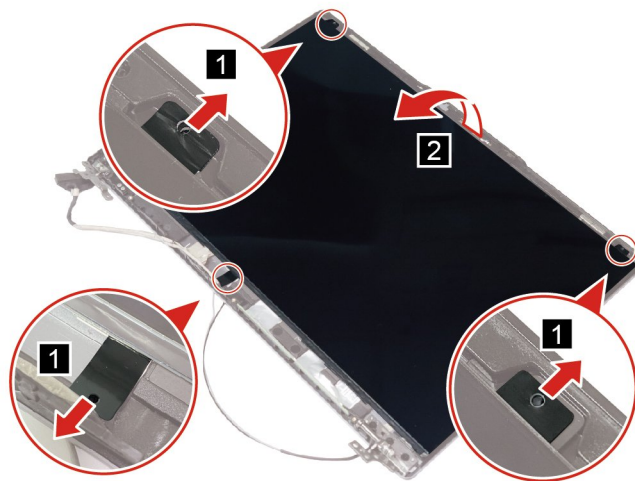
Figure 53. Detach five pieces of stretch-release tape and turn over the OLED panel (for 14-inch models)
