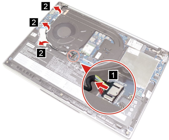
Figure 18. Disconnect the battery pack cable and release the antenna cables
