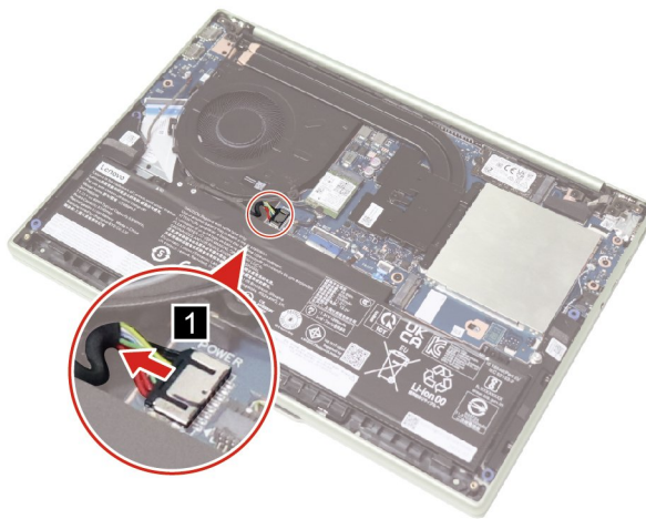
Figure 20. Disconnect the battery pack cable from the system board
