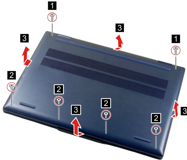
Figure 44. Remove six screws and the lower case
