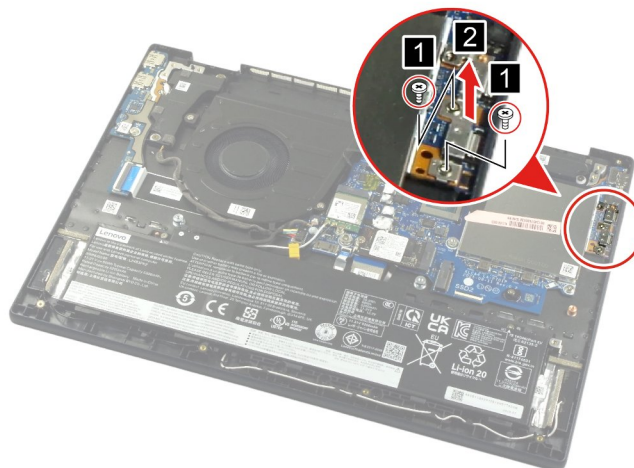
Figure 81. Remove the Type-C bracket
