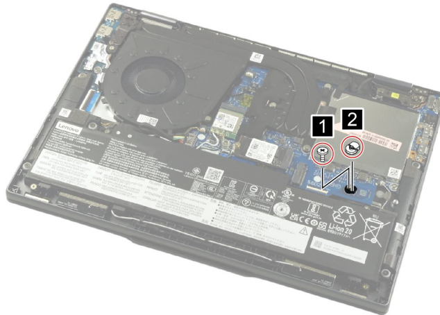
Figure 7. Remove the 2242 trans cover
