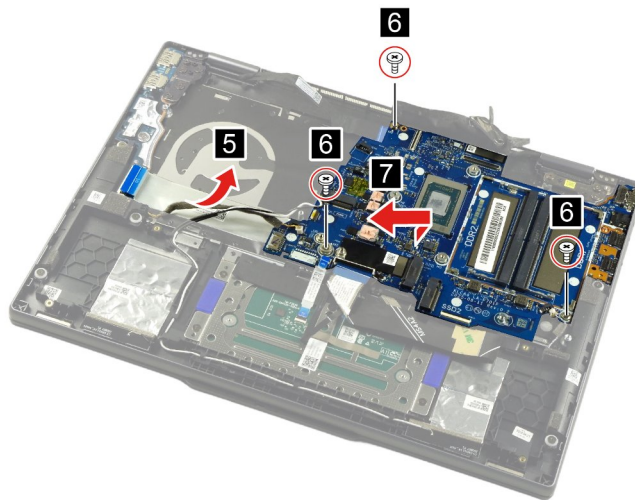
Figure 23. Remove three screws and remove the system board
