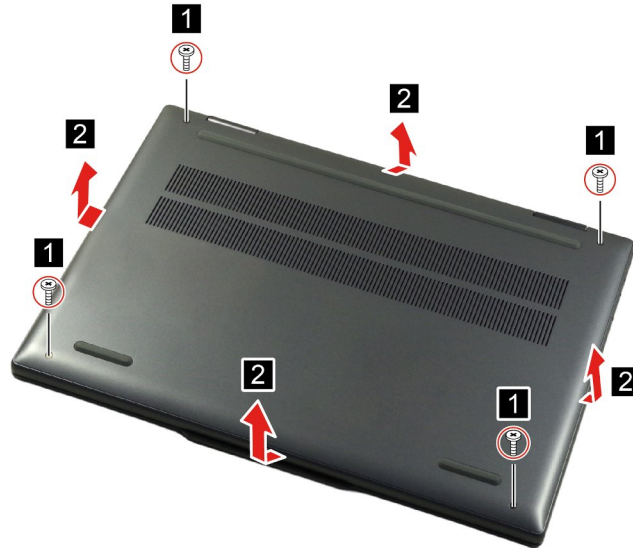
Figure 1. Remove four screws and the lower case
