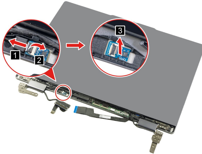
Figure 32. Remove the sensor board
