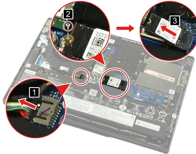
Figure 6. Remove the solid-state drive
