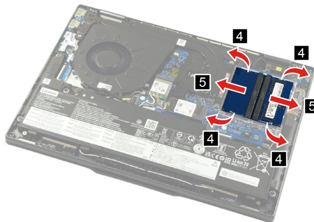
Figure 12. Remove the memory module
