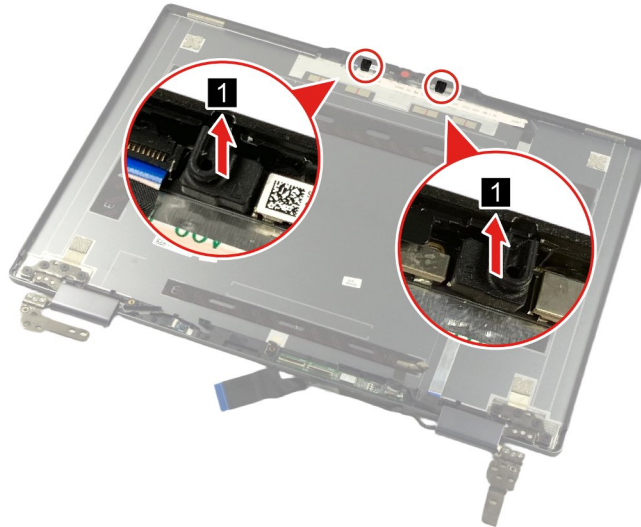
Figure 38. Remove the microphone rubbers
