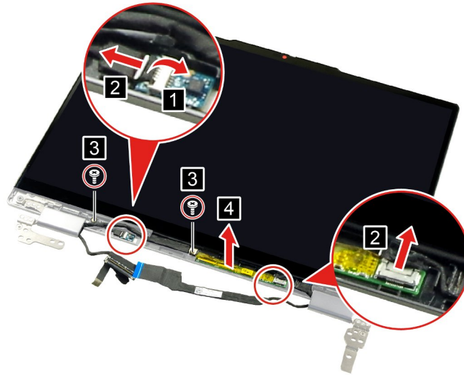
Figure 33. Disconnect the touch board connector and the sensor board connector, remove two screws, and pry up the touch board
