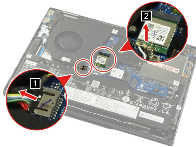
Figure 8. Remove the Wi-Fi card mylar
