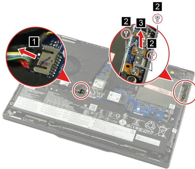
Figure 10. Remove the Type-C bracket
