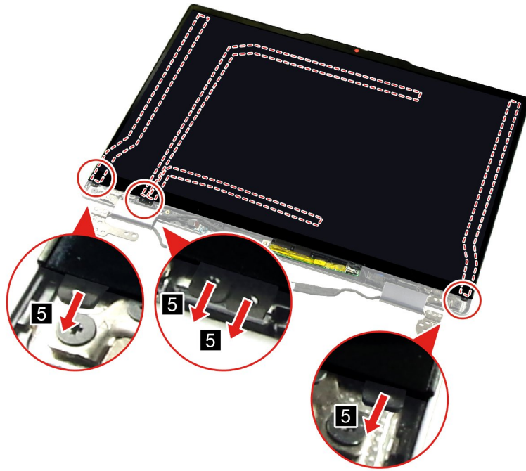
Figure 34. Take out the stretch-release tapes
