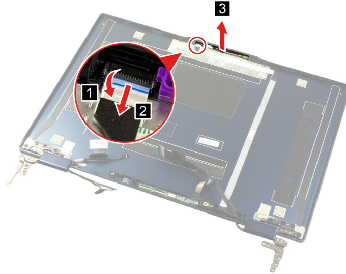
Figure 80. Remove the camera board
