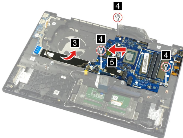
Figure 84. Remove three screws and remove the system board
