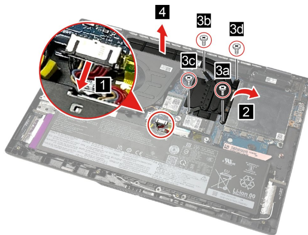
Figure 60. Remove the heat sink (for Intel models)
