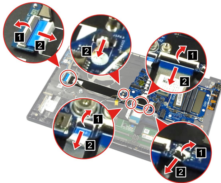
Figure 83. Disconnect the cables
