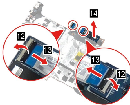
Figure 26. Disconnect the PMIC cable and then remove the PMIC board
