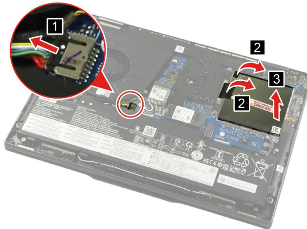
Figure 11. Remove the memory shielding
