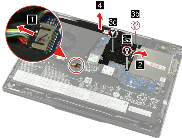
Figure 13. Remove the heat sink (for AMD models)
