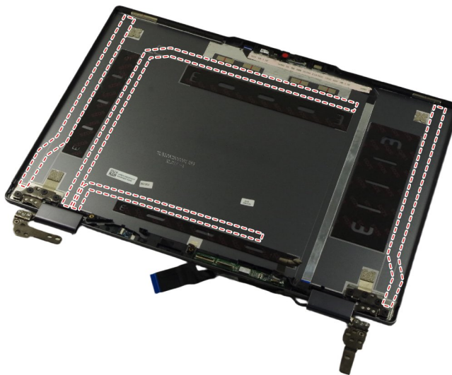
Figure 36. The locations of the stretch-release tapes
