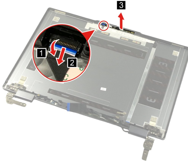
Figure 42. Remove the camera board
