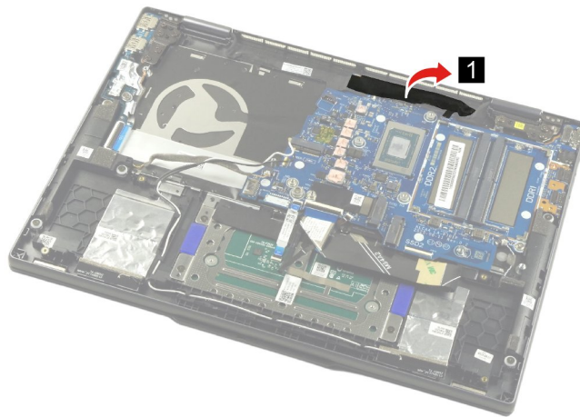
Figure 21. Peel off the MB acetate tape
