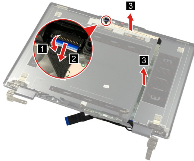
Figure 41. Remove the camera cable
