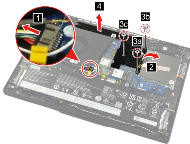
Figure 59. Remove the heat sink (for AMD models)
