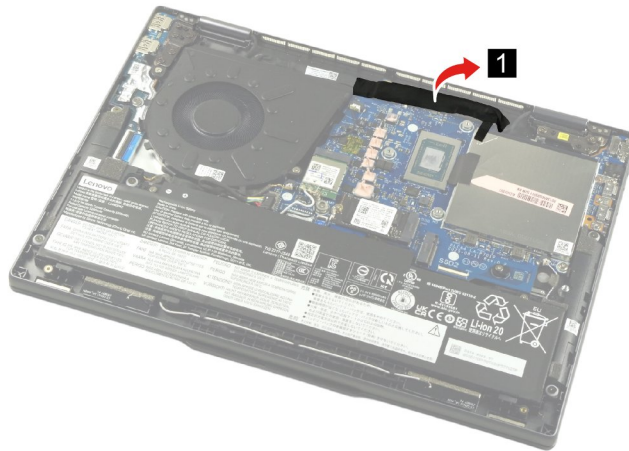
Figure 27. Peel off the MB acetate tape
