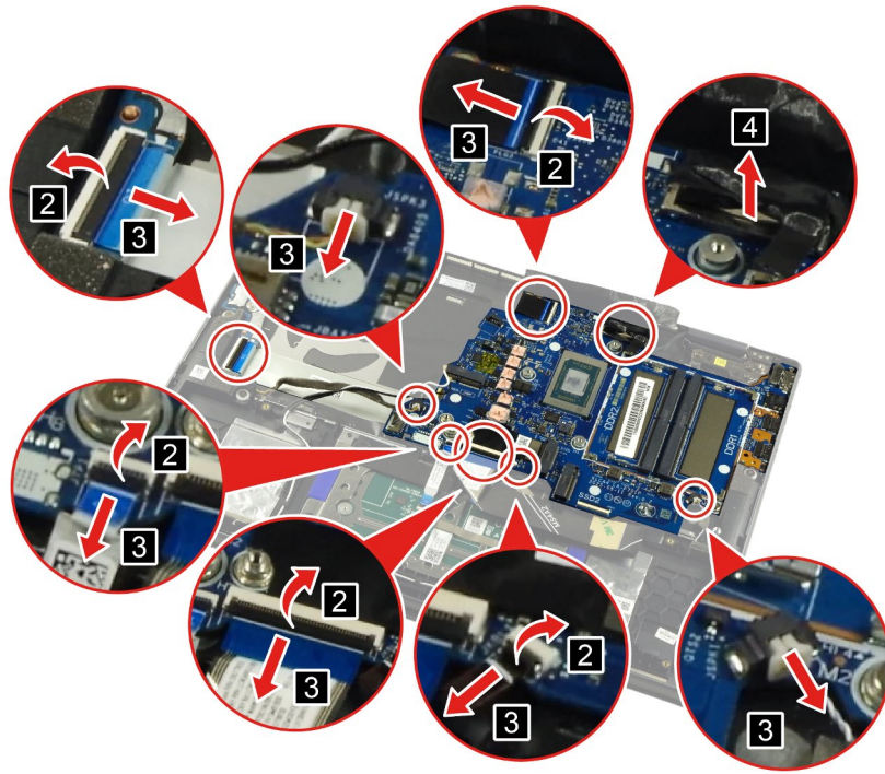
Figure 22. Disconnect the cables
