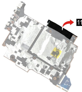
Figure 25. Peel off the MB acetate tape covering the PMIC board and the PMIC cable
