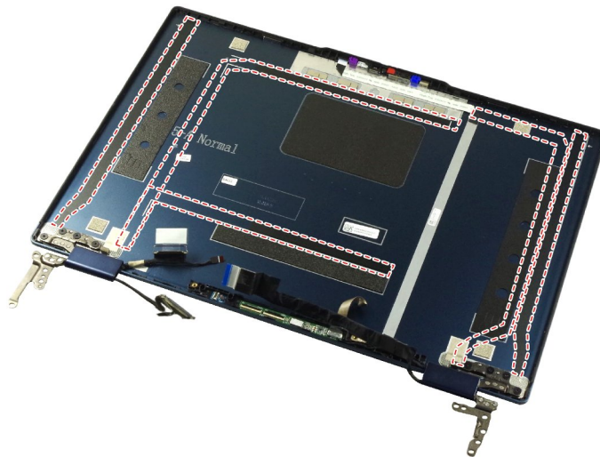
Figure 74. The locations of the stretch-release tapes
