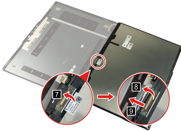
Figure 35. Remove the EDP cable
