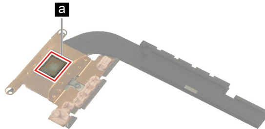
Figure 15. Areas on the heat sink where thermal interface materials should be applied (for AMD models)
