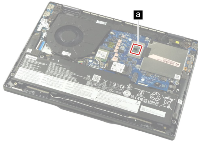
Figure 17. Areas on the system board where thermal interface materials are applied (for AMD models)
