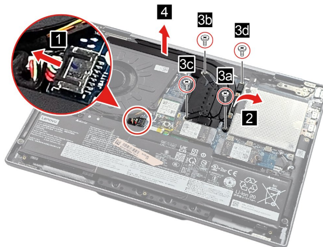
Figure 14. Remove the heat sink (for Intel models)
