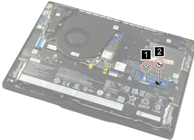
Figure 53. Remove the 2242 trans cover
