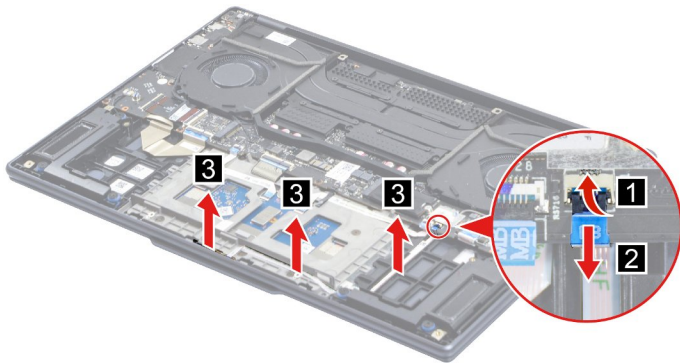
Figure 13. Remove the microphone board with cable
