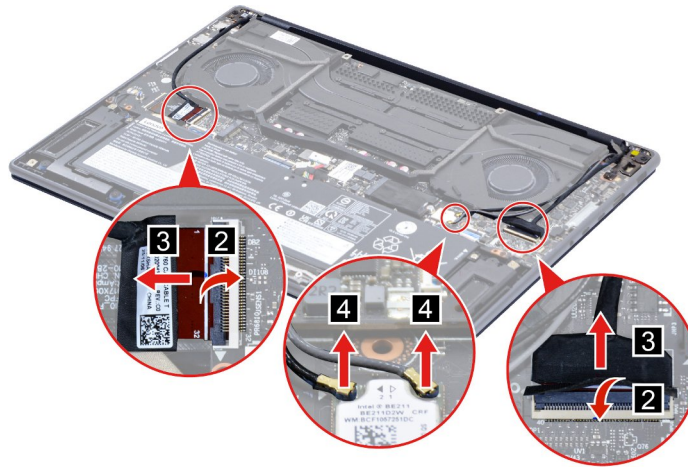
Figure 32. Disconnect cables and connectors
