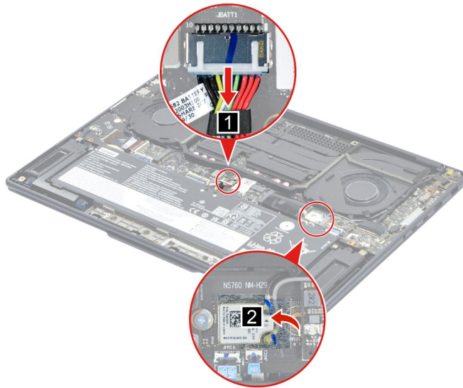
Figure 6. Remove the Wi-Fi card mylar
