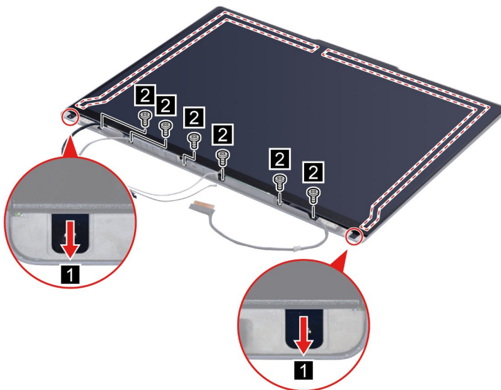
Figure 37. Remove removable tapes and six screws
