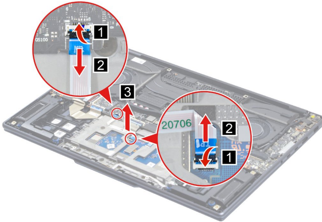
Figure 15. Remove the force pad FFC1
