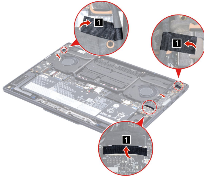
Figure 31. Peel off the tapes and release the cables from cable guides
