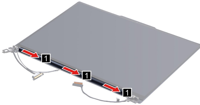
Figure 34. Remove the hinge cover
