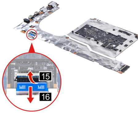
Figure 29. Disconnect the PMIC FFC from the system board
