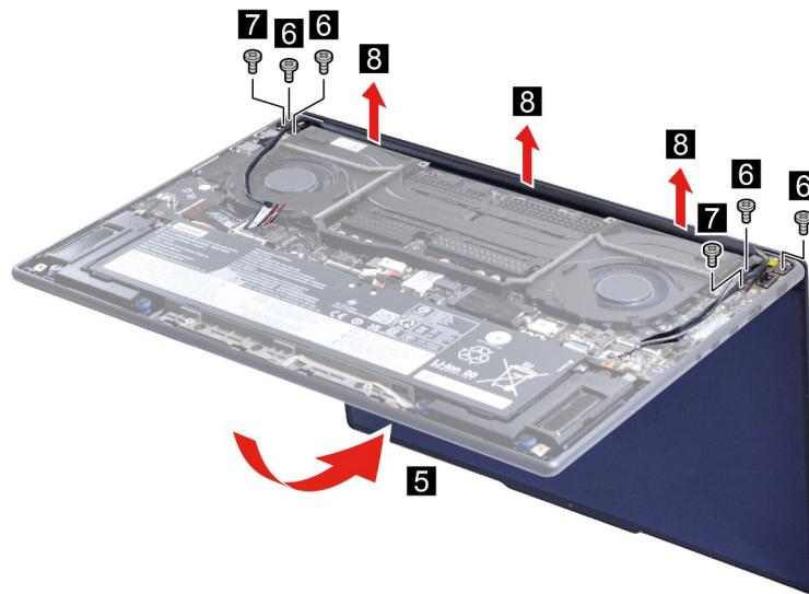
Figure 33. Remove the display assembly
