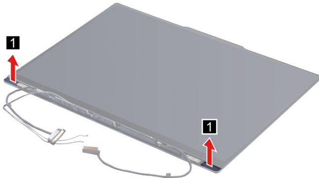
Figure 36. Remove the strip cover
