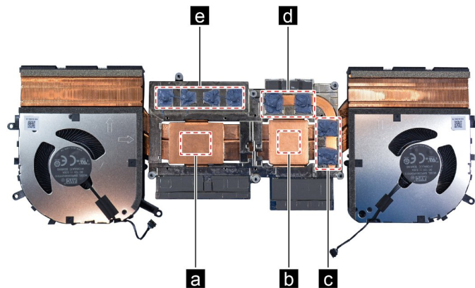
Figure 19. Areas on the heat sink where thermal interface materials should be applied
