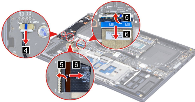
Figure 22. Disconnect the cables
