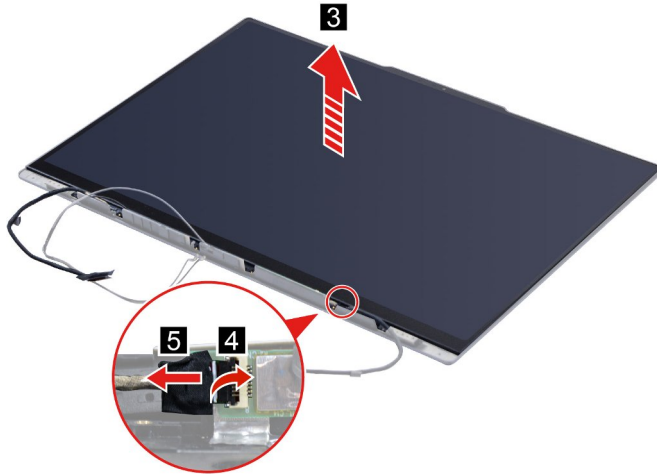
Figure 38. Remove the panel
