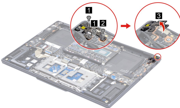
Figure 25. Remove three screws and open the hinge
