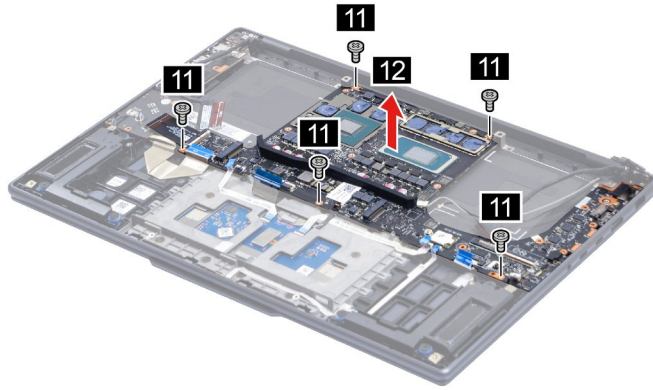
Figure 27. Remove five screws and remove the system board
