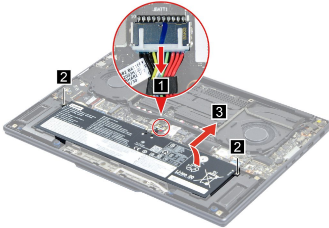
Figure 4. Remove the battery pack
