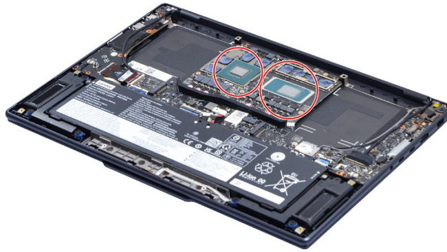
Figure 20. Areas on the system board where thermal interface materials are applied
