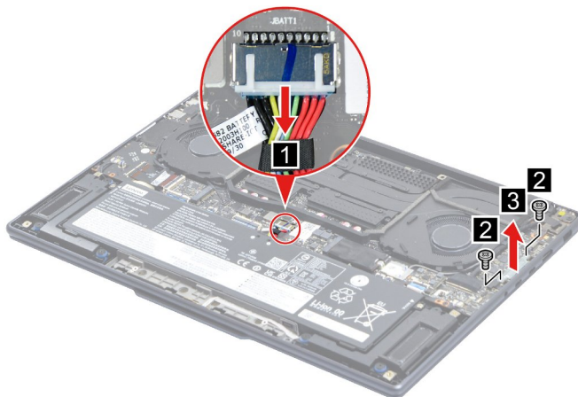
Figure 12. Remove the Type-C bracket
