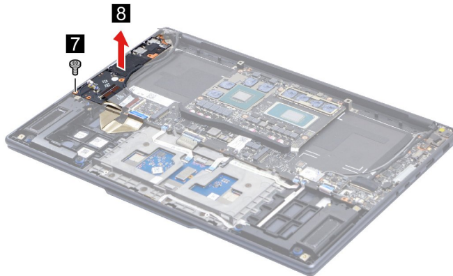
Figure 23. Remove one screw and remove the I/O board
