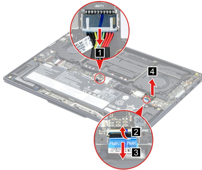
Figure 11. Remove the PMIC board
