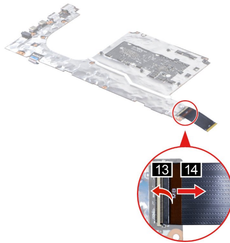
Figure 28. Disconnect the I/O FPC from the system board
