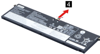
Figure 5. Remove the battery pack cable
