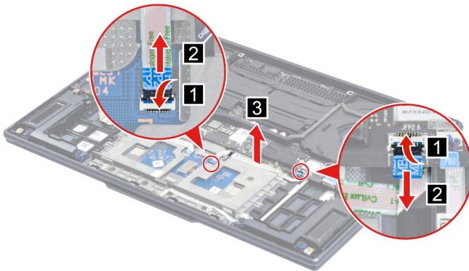
Figure 16. Remove the force pad FFC2
