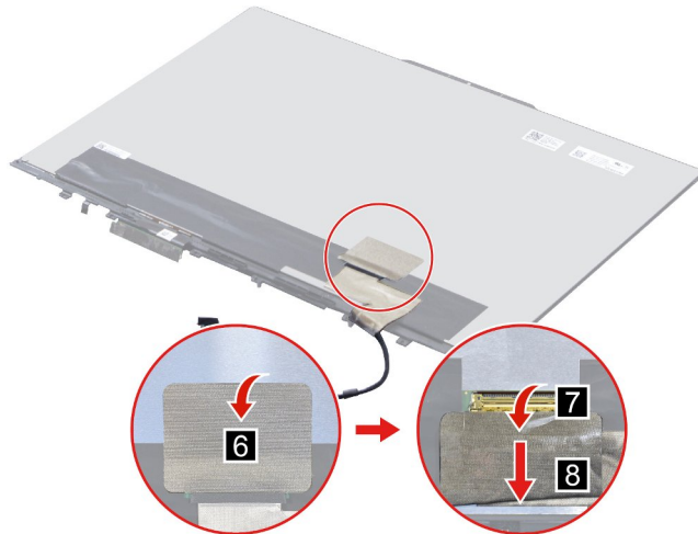
Figure 39. Remove the EDP cable from the panel
