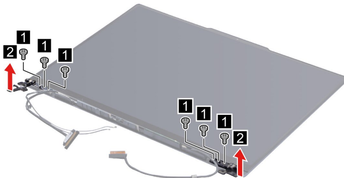
Figure 35. Remove the hinges
