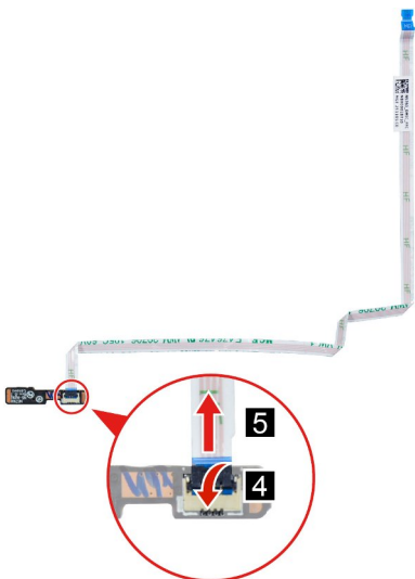
Figure 14. Remove the microphone cable
