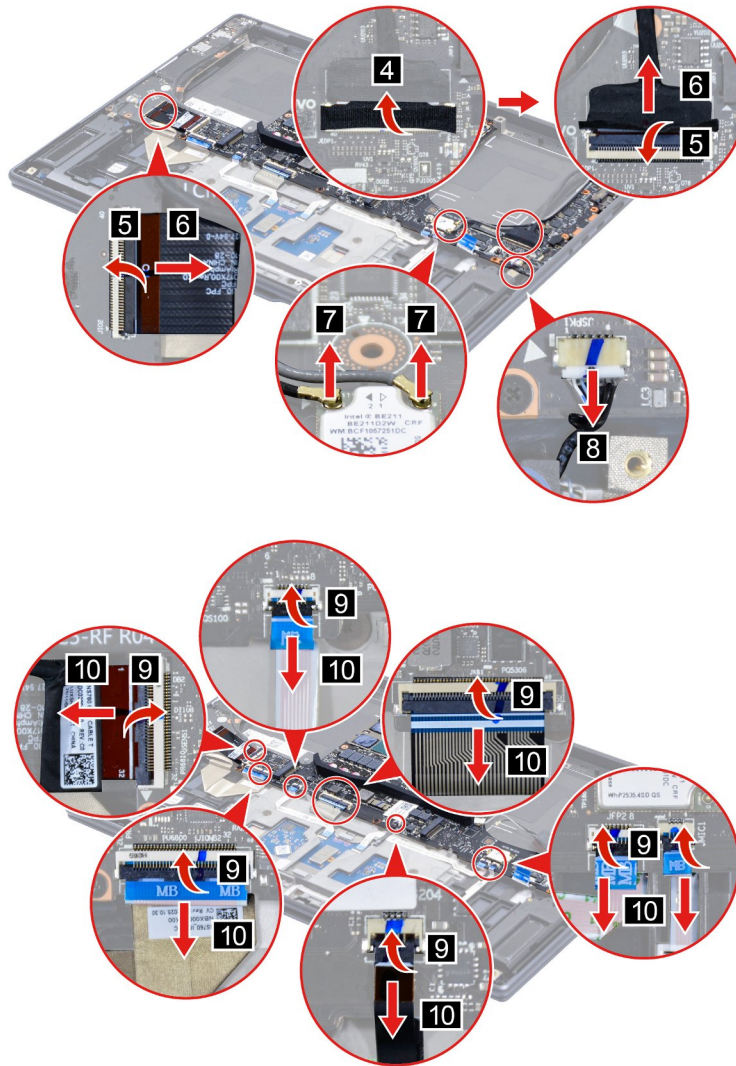
Figure 26. Disconnect cables
