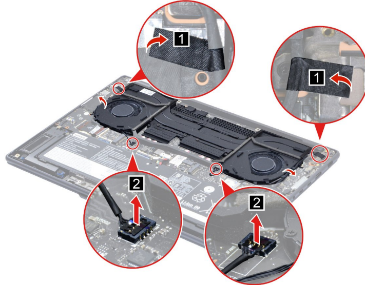
Figure 17. Disconnect two fan cables from the system board
