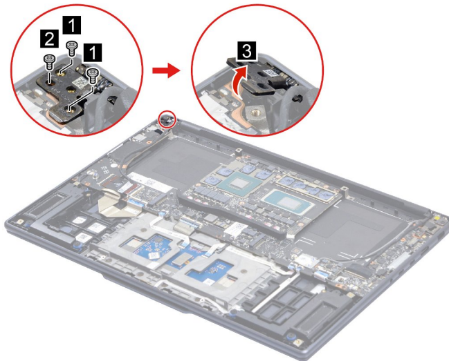
Figure 21. Remove three screws and open the hinge
