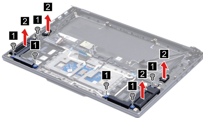
Figure 30. Remove the speakers
