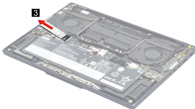
Figure 10. Remove the 2280 solid-state drive
