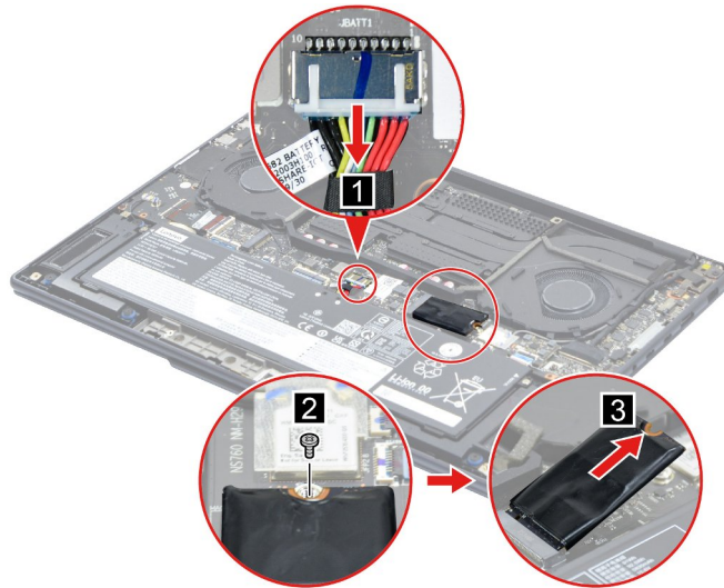
Figure 7. Remove the 2242 solid-state drive
