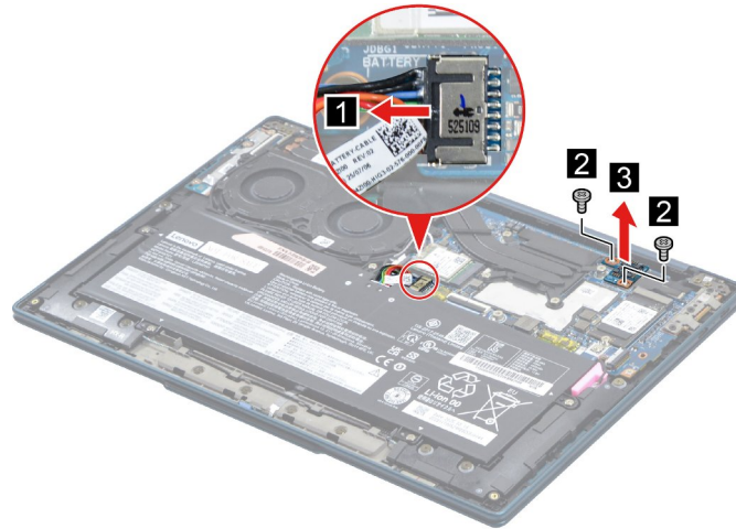
Figure 16. Remove two screws and remove the PMIC board
