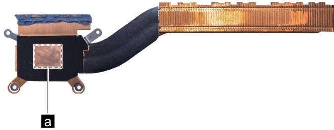
Figure 11. Areas on the heat sink where thermal interface materials should be applied
