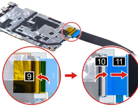
Figure 21. Disconnect the I/O board cable from the system board
